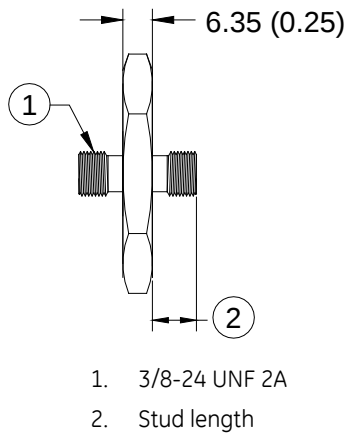
Figure 1: Hex Plate Stud for "A" Options 02, 03, 05, 17, 18, and 23.
