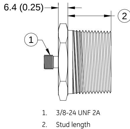
Figure 3: Hex Stud for "A" Options 06 Through 11
