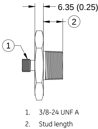
Figure 2: Hex Plate Stud for "A" Option 04
