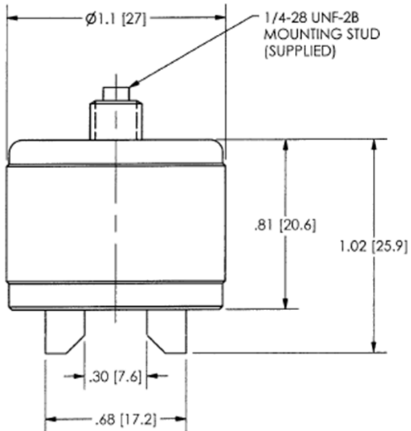
Figure 9: Magnetic Base Dimensional Drawing
