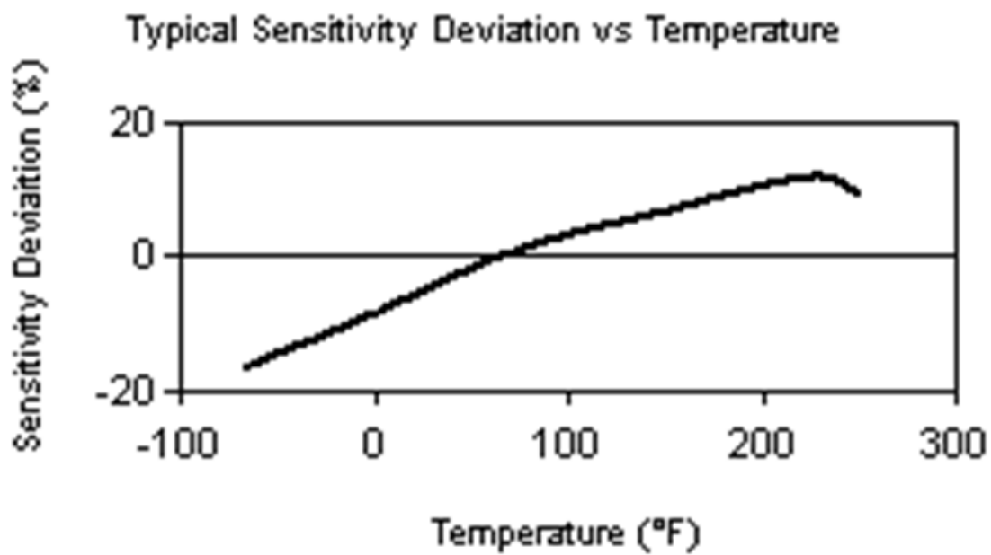
Figure 7: Temperature Sensitivity Curve
