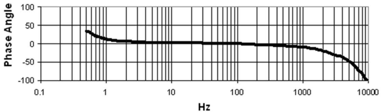
Figure 4: 200350 Accelerometer Phase
