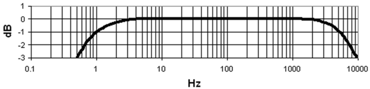
Figure 3: 200350 Accelerometer Frequency Response
