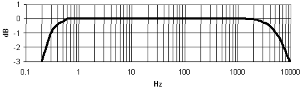
Figure 5: 200355 Accelerometer Frequency Response
