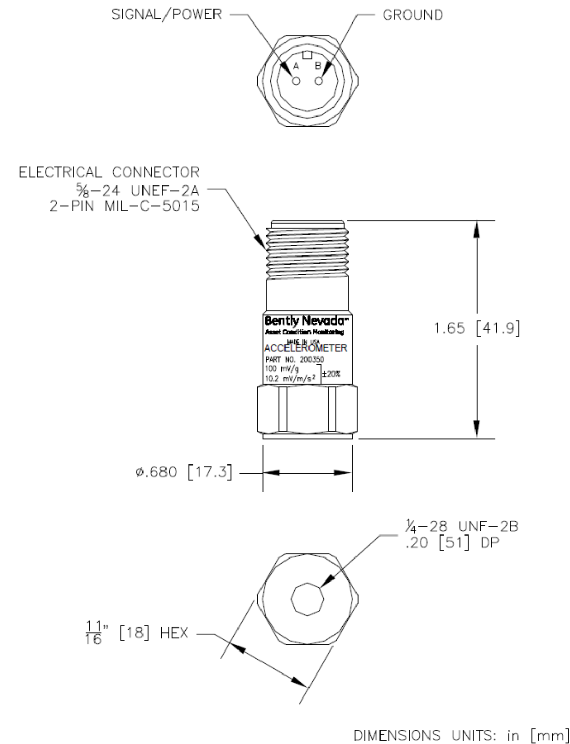
Figure 1: 200350 Accelerometer Dimensional Drawing
