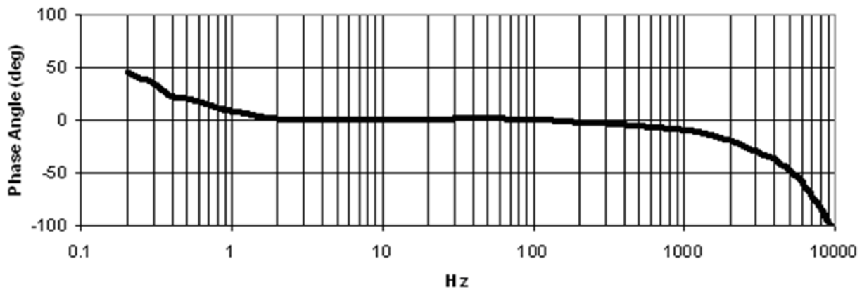
Figure 6: 200355 Accelerometer Phase
