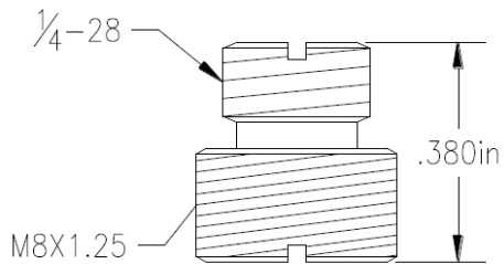
Figure 8: Mounting Stud Dimensional Drawings
