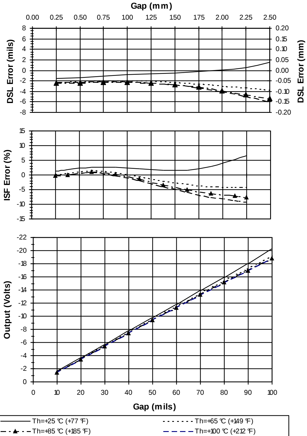
Figure 3: Typical 3300 XL 8mm 9m Proximity Sensor with 8m Extension Cable at T_h (Probe is at 25 ^{\circ}\text{C} )
