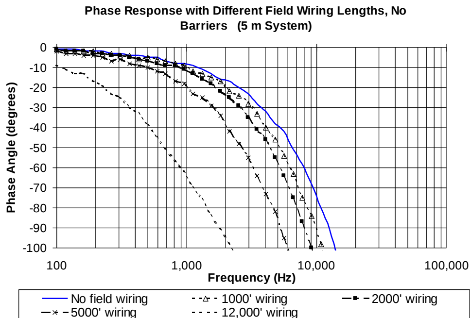
Figure 7: Phase Response, Typical 3300 XL 8mm 5m or 1m System with Varying Lengths of Field Wiring Attached, No Barriers
