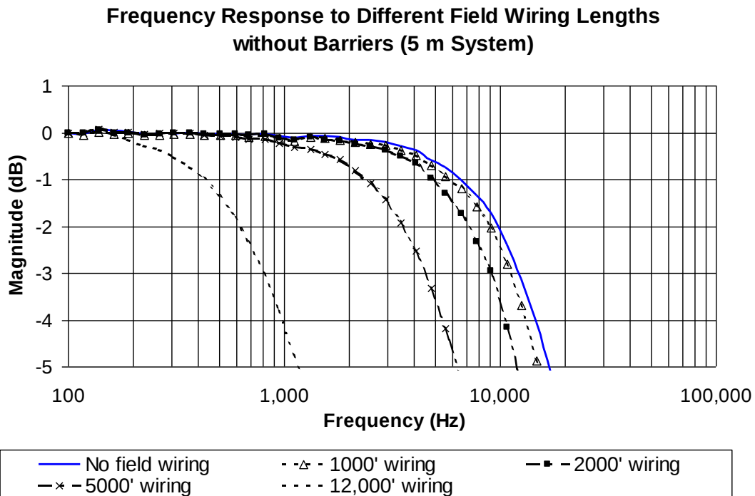
Figure 6: Frequency Response, Typical 3300 XL 8mm 5m or 1m System with Varying Lengths of Field Wiring Attached, No Barriers
