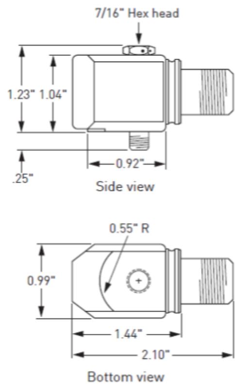
Figure 2: AS3100S2-Z0 dimensions
