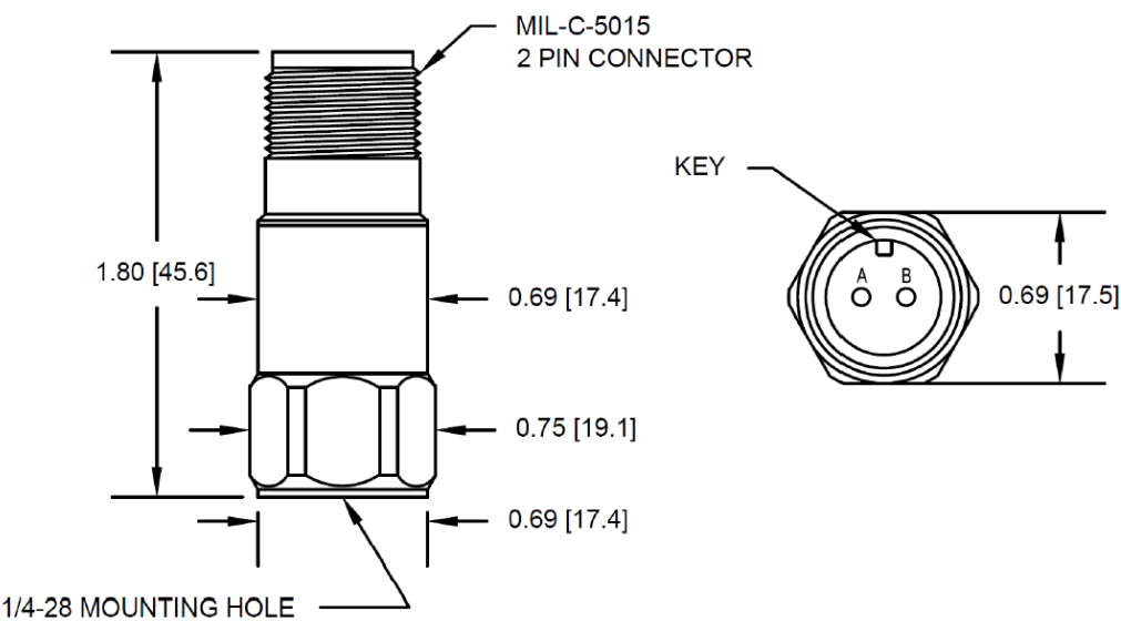
Figure 1: AM3100T2-Z2 dimensions
