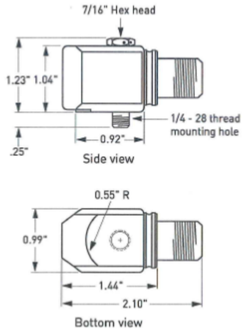
Figure 5: AP3500T2-Z1 dimensions
