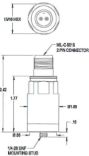
Figure 5: AP3500T2-Z1 dimensions
